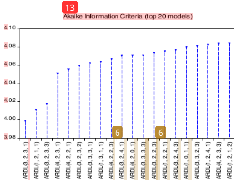
Figure 3.1 Optimum Lag Test
